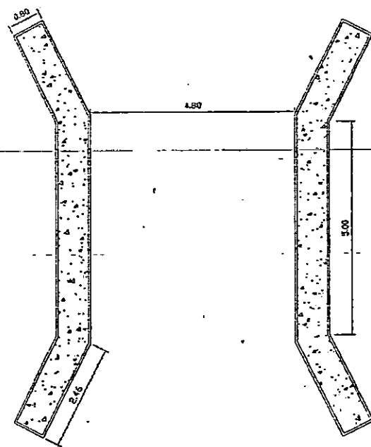
FOUNDATION PLAN
