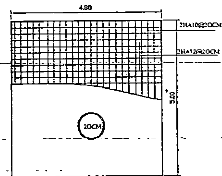
REINFORCEMENT PLAN
